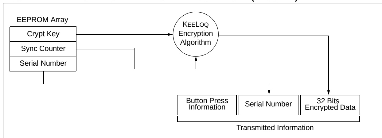
FIGURE 1-2: BUILDING THE TRANSMITTED CODE WORD (ENCODER)
