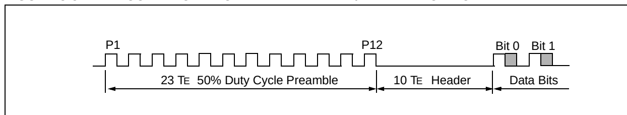
FIGURE 8-3: CODE WORD FORMAT: PREAMBLE/HEADER PORTION
